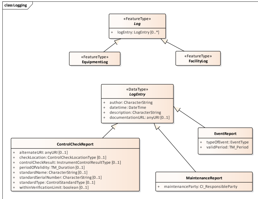
Figure 2 Log and LogEntry model
