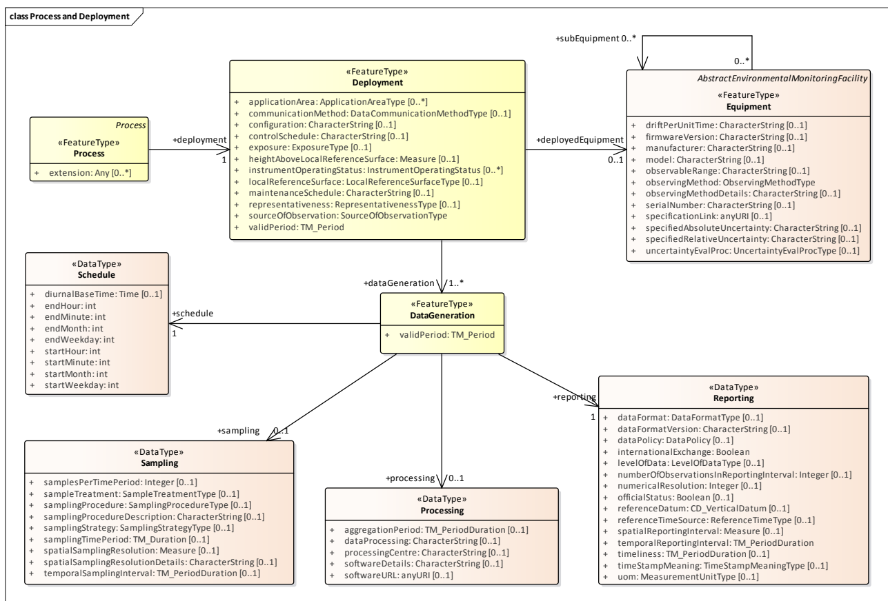
Figure 4 Showing the Process, Deployment and relationships
