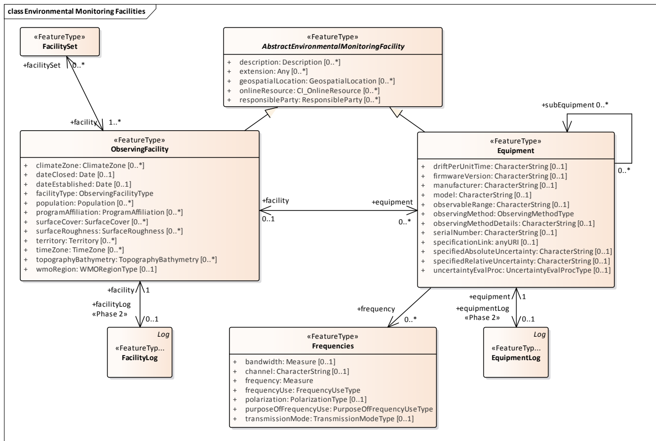
Figure 1 ObservingFacility and Equipment
