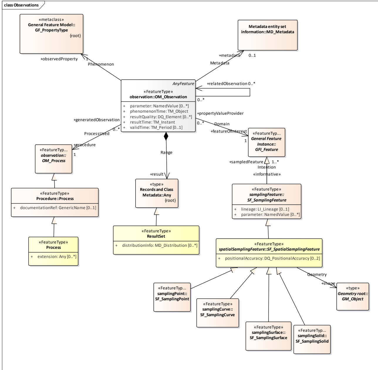
Figure 3 The profiling of O&M in WMDR
